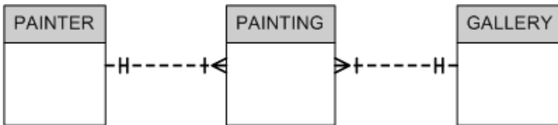
FIGURE P2.10b The UBA Relational Diagram
