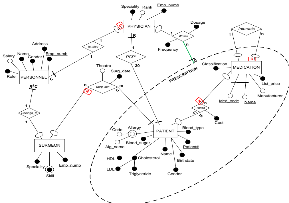
Deletion constraints enclosed in a box (highlighted in red) reflect erroneous/conflicting deletion (business) rules. A few different ways of correction are possible. Once such correction is shown in the next ER diagram
