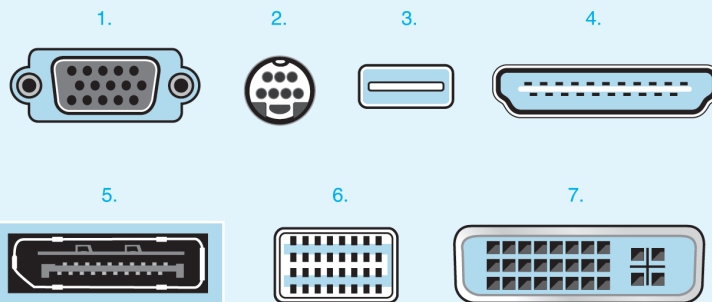
Figure 1.55 Video ports
