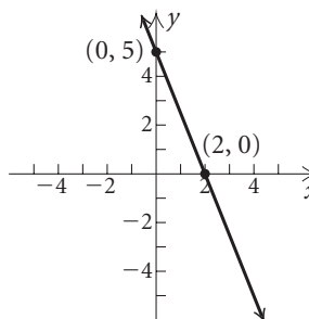
10 - 5x = 2y
